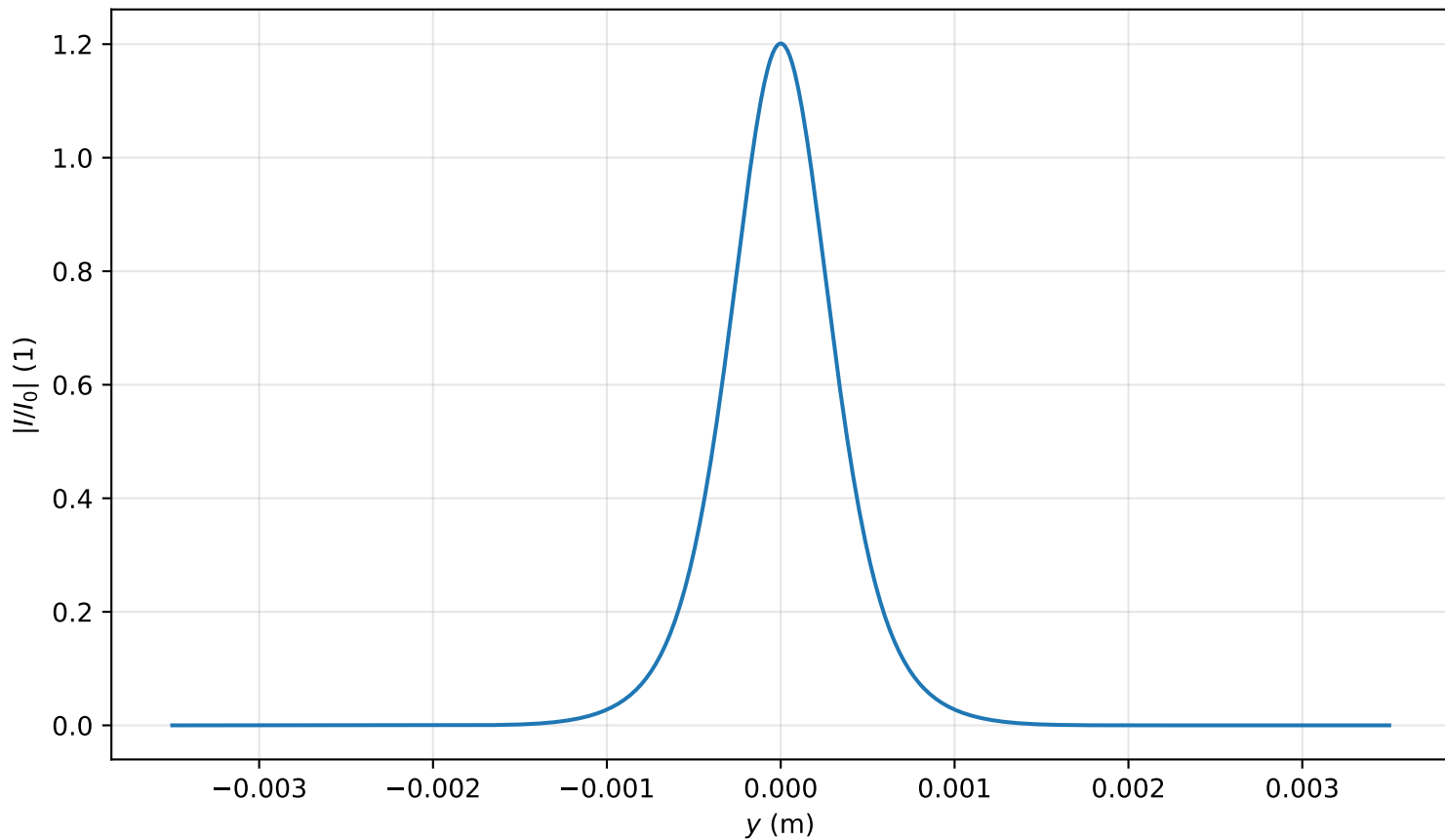
Intensity profile I(x=0, y, z=1.433)/I_0 , P_{in}=0.7P_{cr} , artificial time
